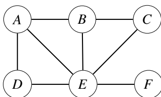
Figure 1: An undirected graph on six vertices. To interpret this as the transition diagram of a Markov chain, view each undirected edge as a pair of directed edges, one in each direction. Transition probabilities for all edges out of a given vertex are equal.
